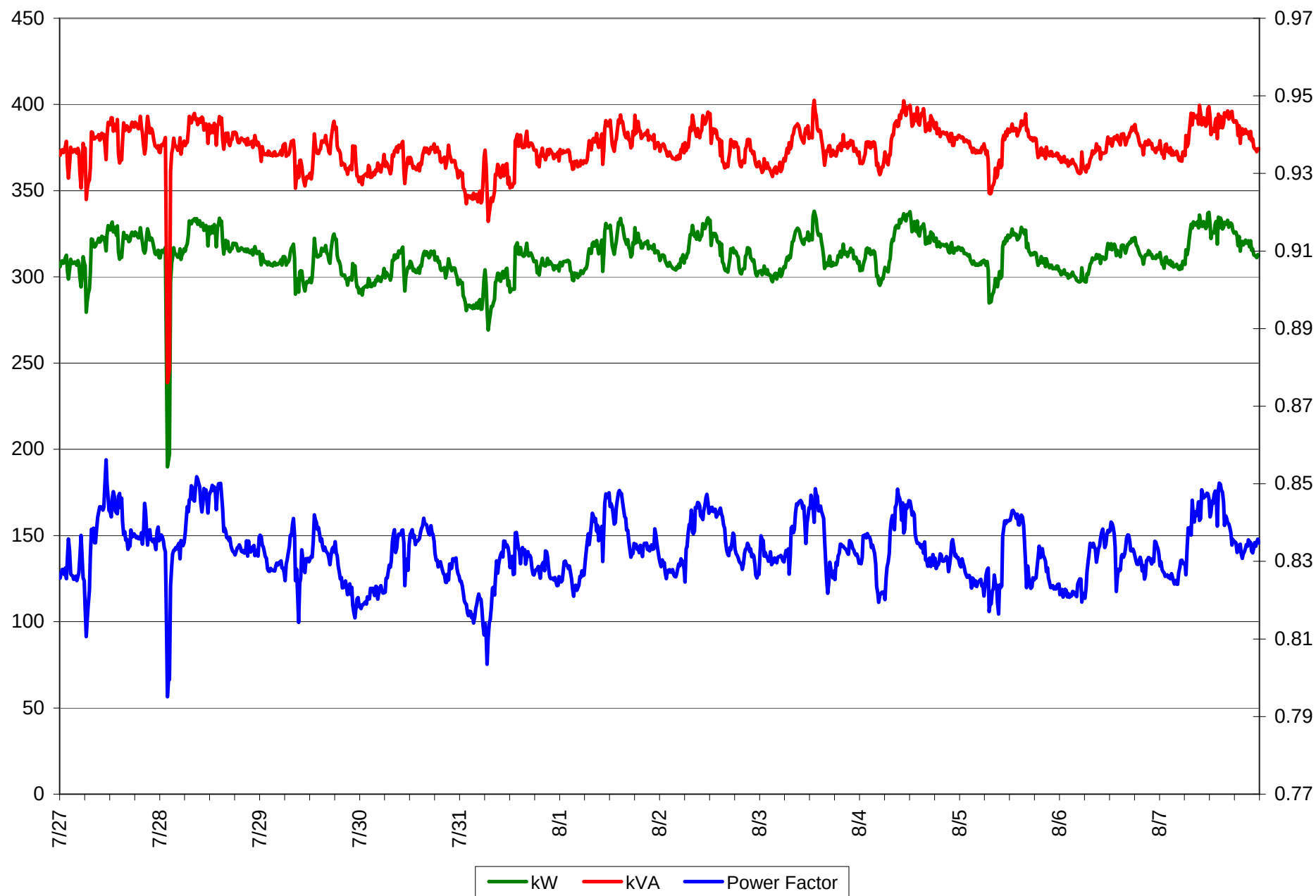
Total kW, kVA & Power Factor for Hospital Emergency Loads
